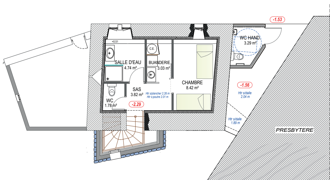
PLAN MEZZANINE
